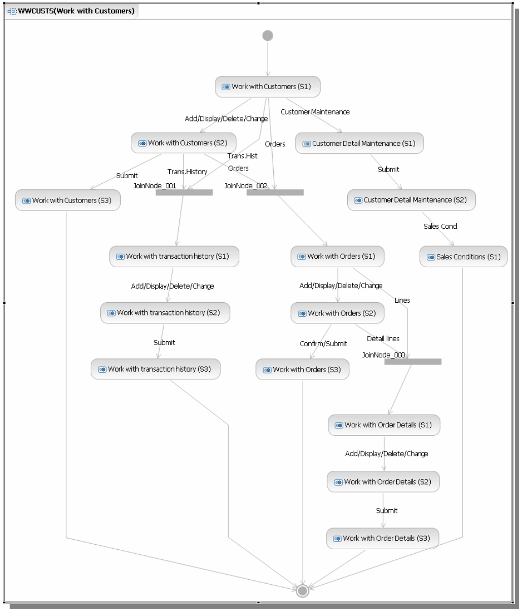
Figure 14 – Activity Diagram
